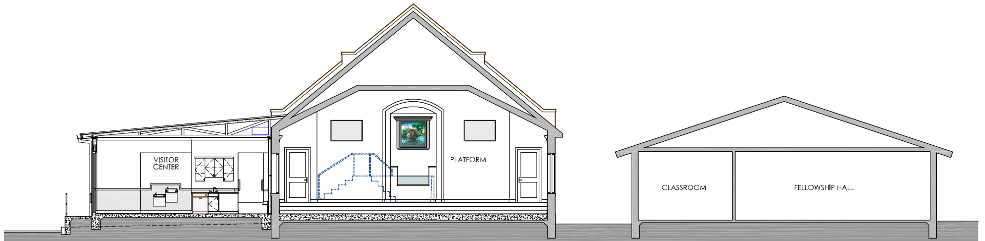
CROSS SECTION
