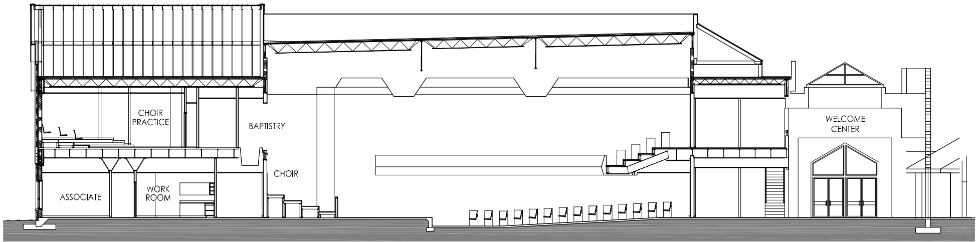
CROSS SECTION
